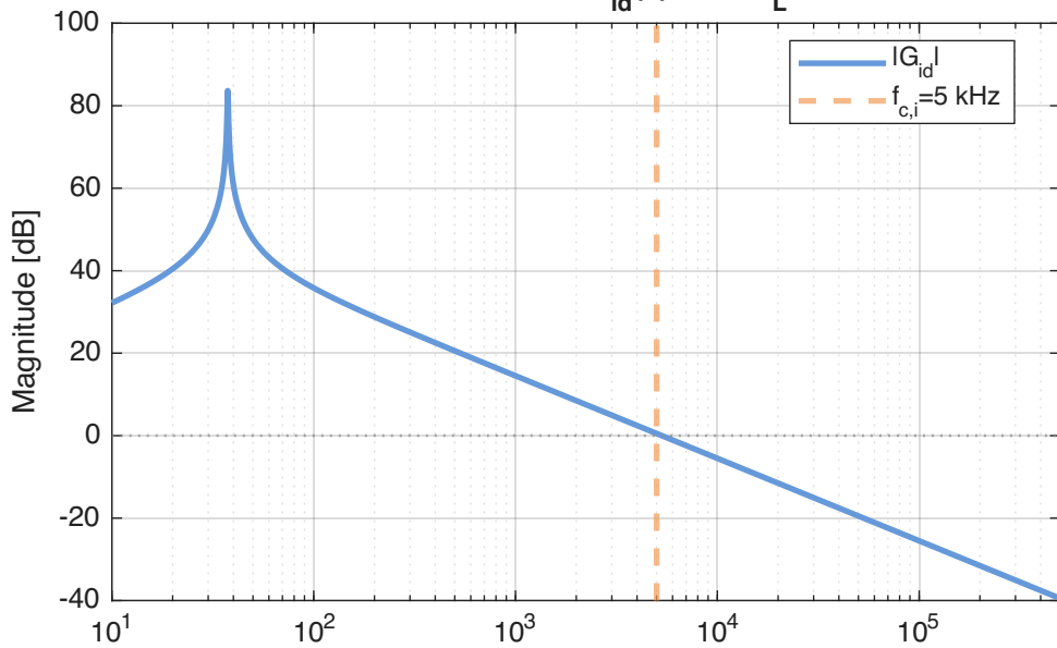
Current Plant G_{id}(s) : d \rightarrow i_L
